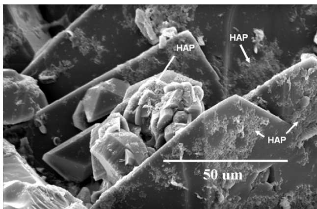
Figure 4 COM, COD and HAP crystal formation (arrows) on post-ESWL COD renal calculi fragments following a 192 h incubation in normocalciuric (3.75 mM) and normoocaluric (0.28 mM) synthetic urine (pH = 6.5).
